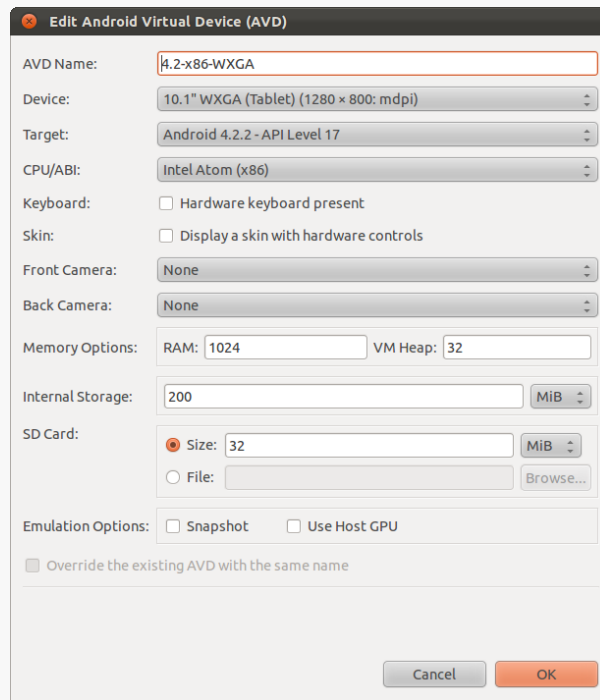
Figure 479: New AVD Configuration Editor, Showing “Use Host GPU” Option
