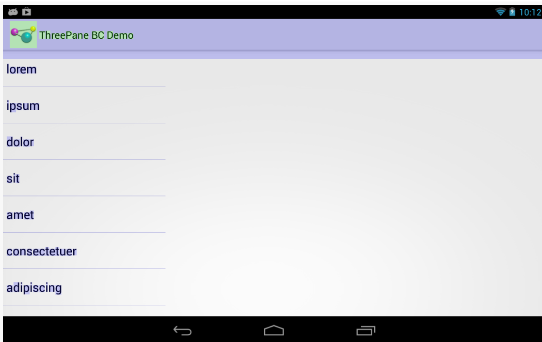
Figure 514: Three-Pane Demo, As Initially Launched, Showing Overdraw
