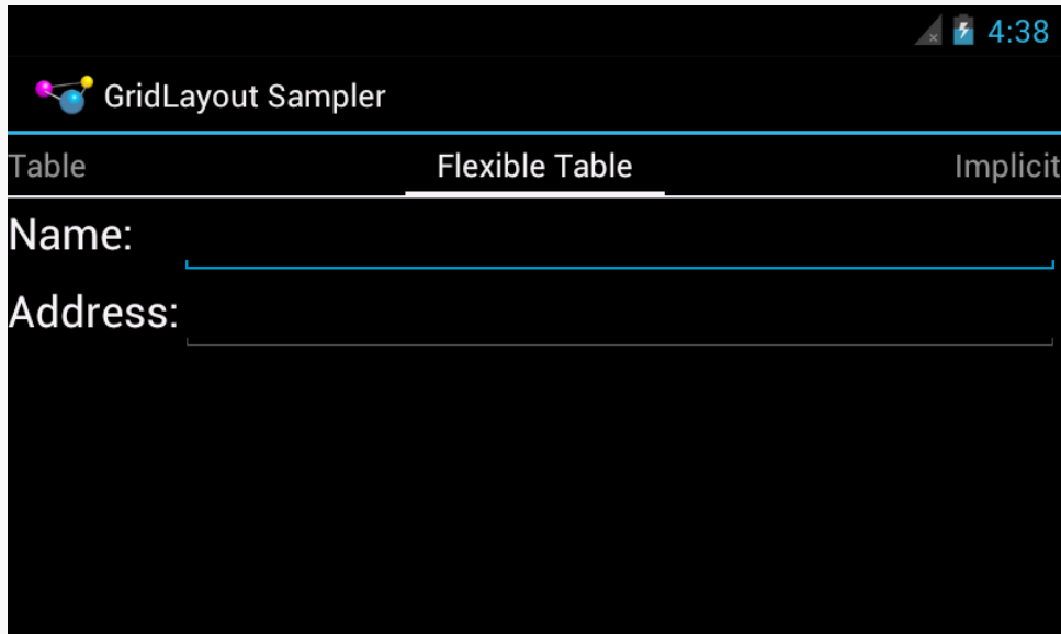
Figure 226: Table Using GridLayout, in Landscape, on a 4.0.3 Emulator
