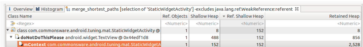
Figure 533: The GC roots holding onto an activity
