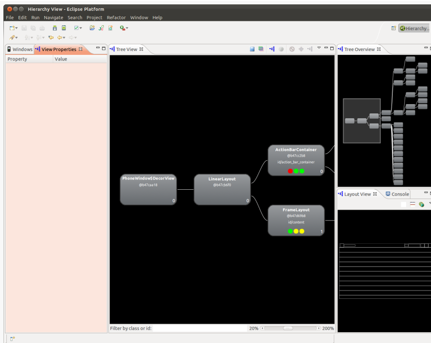
Figure 485: Hierarchy View, in Eclipse, Showing an Activity
