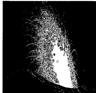
Molten lava ejected from the summit vent of Stromboli volcano.
