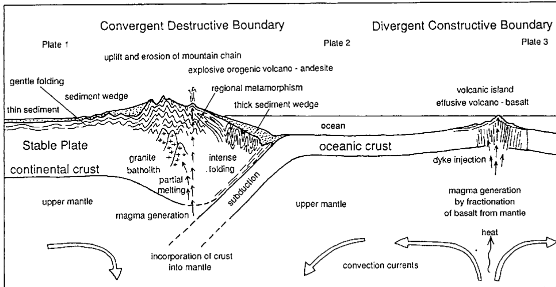
Plate boundary processes
