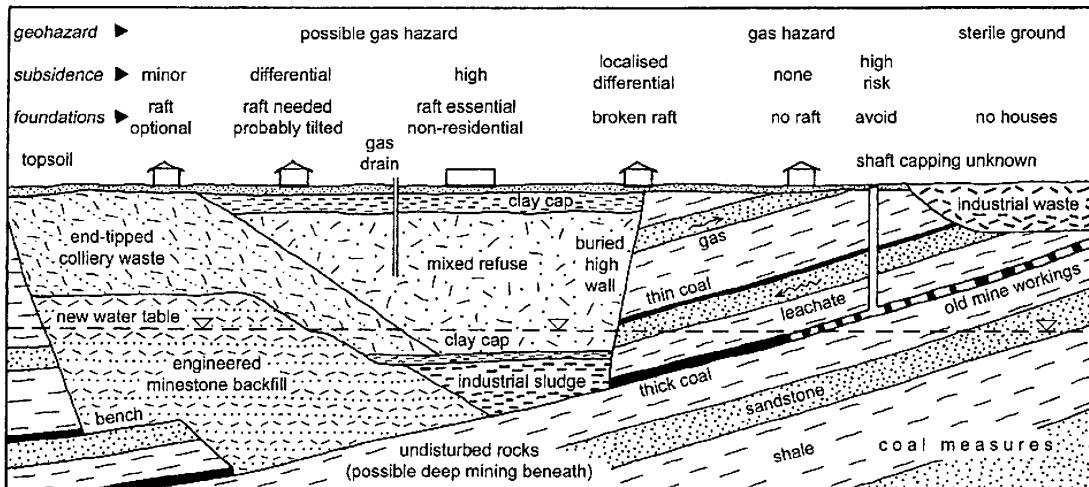
Varying conditions on brownfield land with past mining and landfill, and the state of houses built on rafts.
