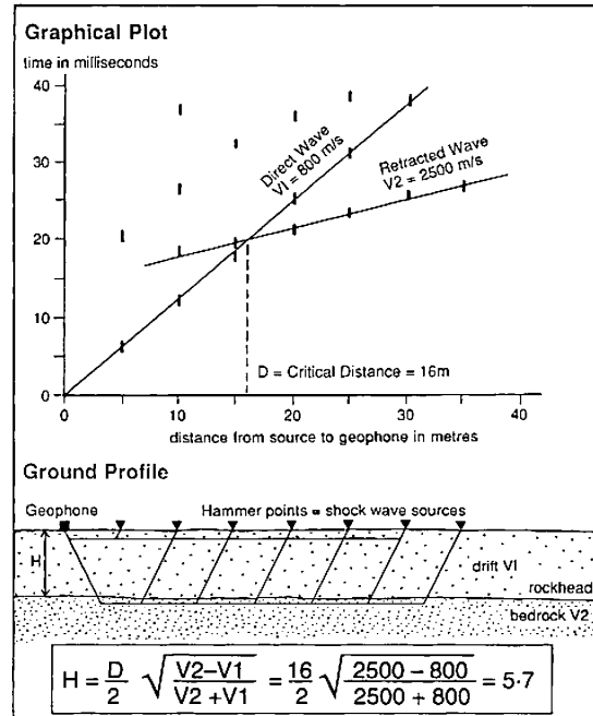
Seismic profile over alluvium above mudstone
