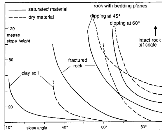
Influence of slope height on stable slope angle
