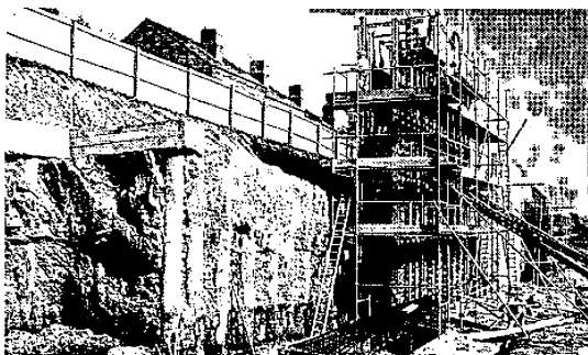
Retaining wall under construction with frontal toe and shear key beneath for new road cut in Derbyshire. Exposed bored piles provided temporary support.
