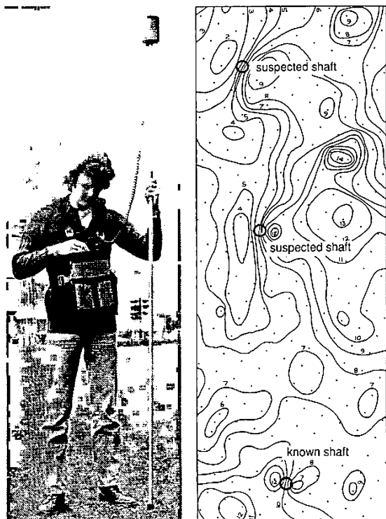
Proton magnetometer and map of a magnetic survey on a site in the Derbyshire coalfield. Stations are on 3 m grid; contours are at 100 nT intervals above a base of 48 000 nT. Dipole anomalies lie over one known shaft and indicate the location of two more shafts
