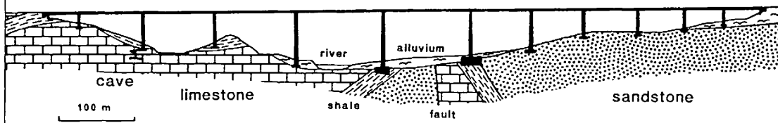
Remouchamps Viaduct
