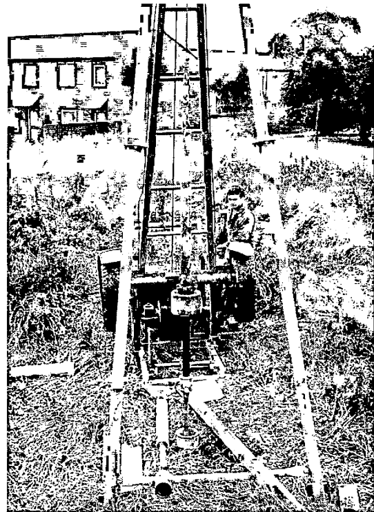
Light percussion rig sampling soils to a depth of 10 m for a construction project in Derbyshire
