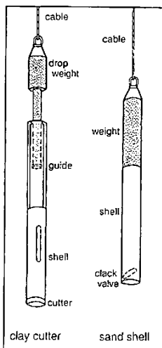
Alternative shells for light percussion drills
