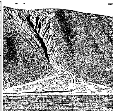
Gully erosion produces new sediment, that builds a steep alluvial fan
