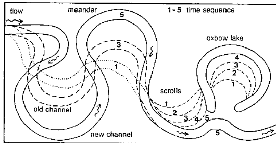
Development of river meanders
