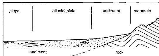
Profile through the typical desert landform zones
