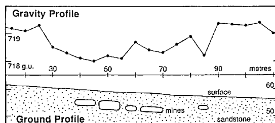
Gravity surveys over sand mines in Nottingham
