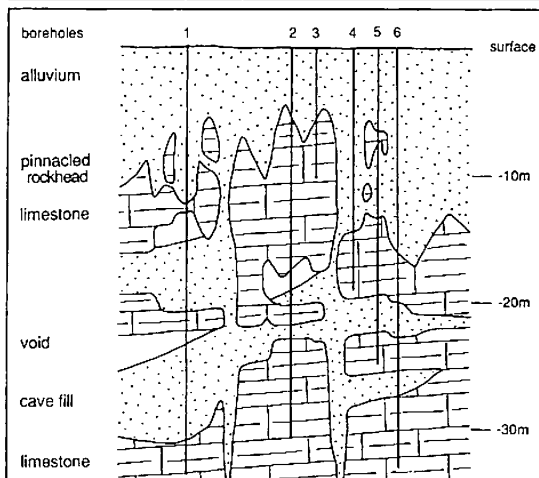
Boreholes on a site in Kuala Lumpur, Malaysia, with an interpreted geological profile reflecting solution along fissures in the massive limestone
