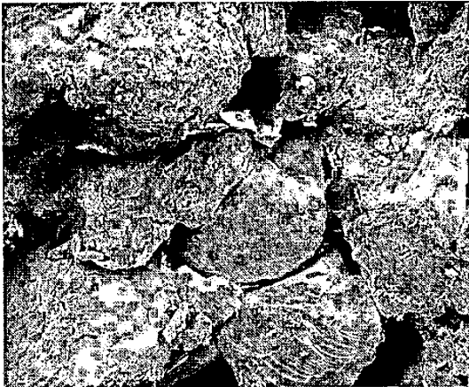
Electron microscope view of sandstone with quartz grains and weak flaky clay mineral cement. An original partial calcite cement has been removed by weathering.
