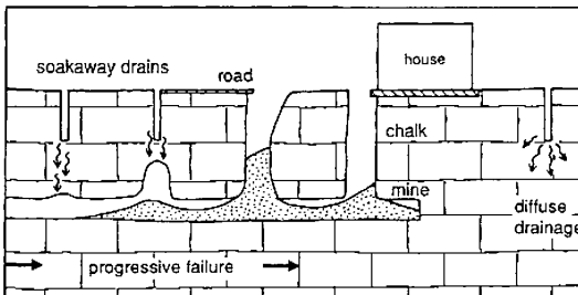
Failures beneath roads in Bury St Edmunds, due to chalk liquefaction between soakaway drains and old mines.
