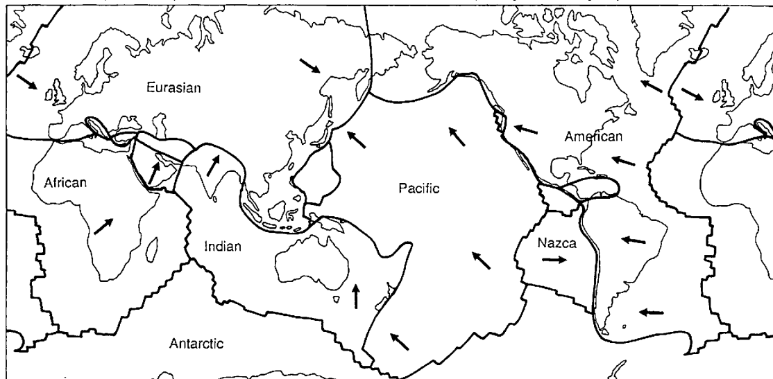
The world's major crustal plate, with arrows to show relative movement (mostly a few cm/year)
