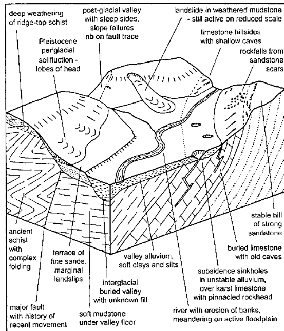
A total geological model for an upland site that was influenced by variations in the Quaternary climate.
