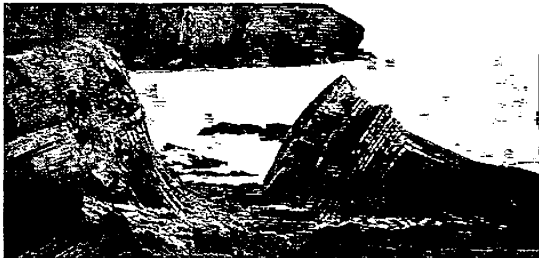
Folded rocks exposed along the South Wales coast
