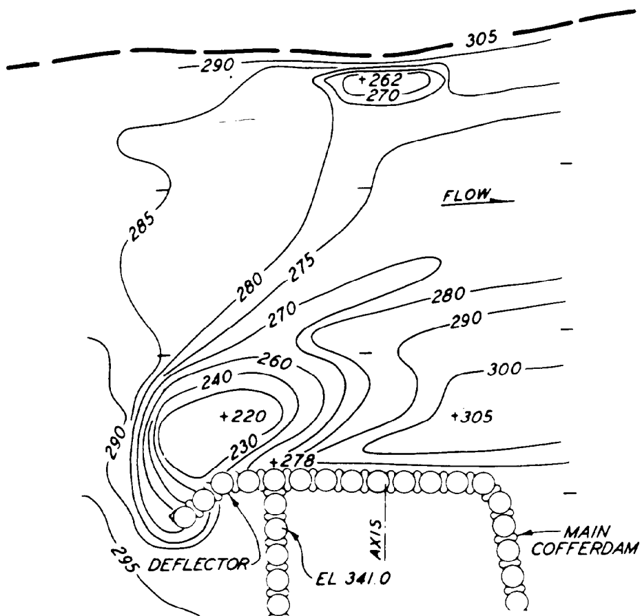
Figure 11-1. Typical scour pattern with deflector
