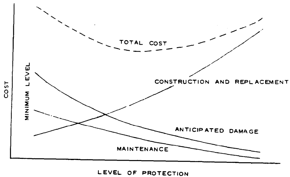
Figure 14-2. Project cost curves
