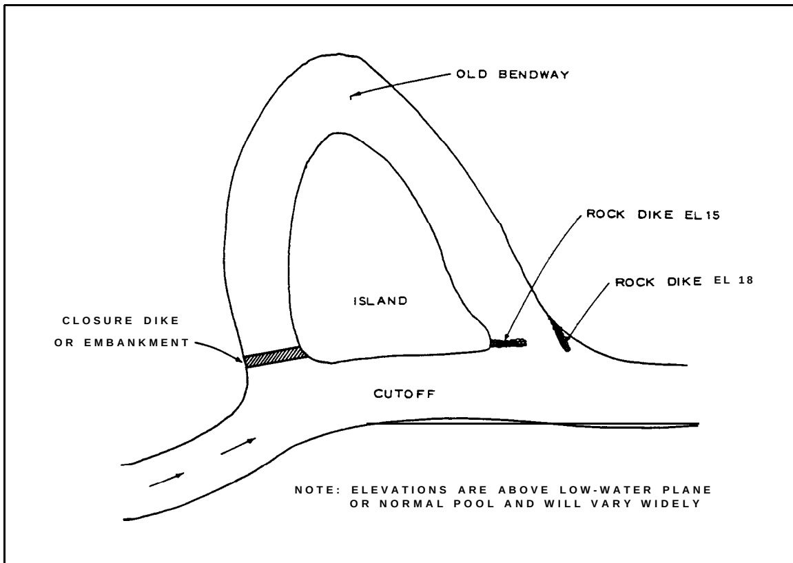
Figure 7-l. Cutoff-old bendway used for harbor or recreation
