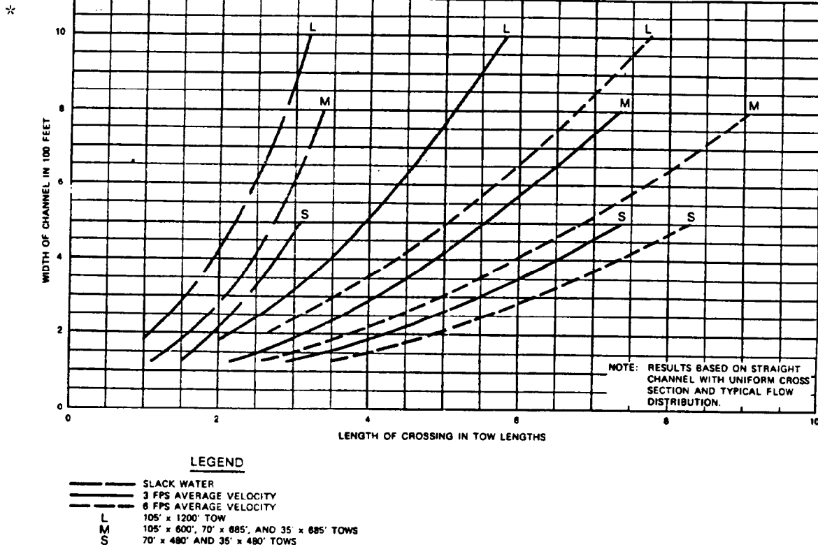
Figure 4-1. Length of channel required between alternate bends ☆
