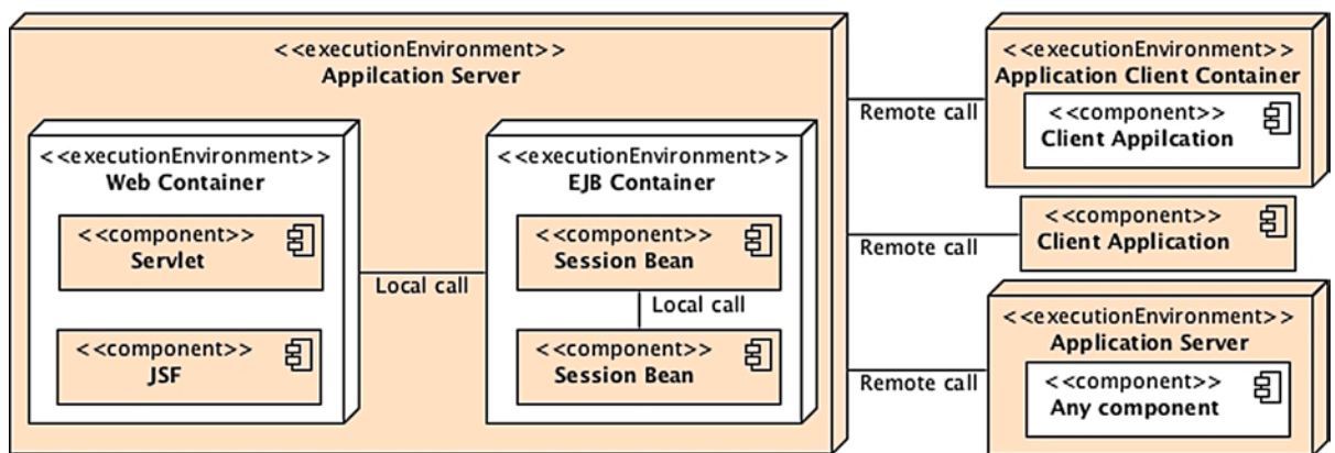
Figure 7-3. Session beans invoked by several types of client
