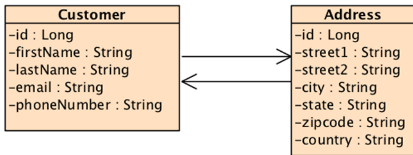
Figure 5-12. A bidirectional association represented with two arrows
