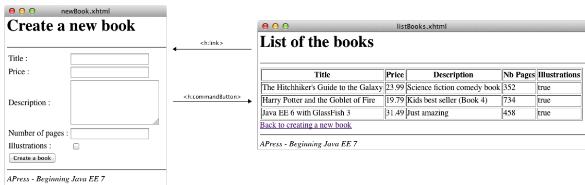
Figure 11-5. Navigating between newBook.xhtml and listBooks.xhtml
