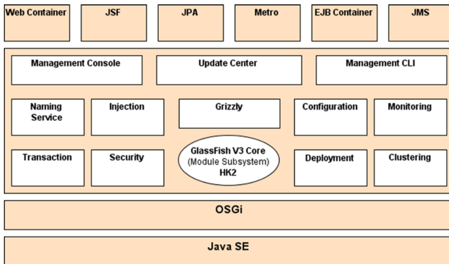
Figure A-10. GlassFish v4 architecture
