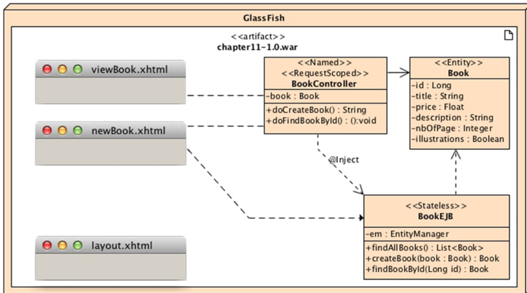
Figure 11-9. Pages and classes involved in the web application
