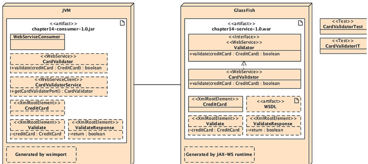
Figure 14-6. Putting It All Together
