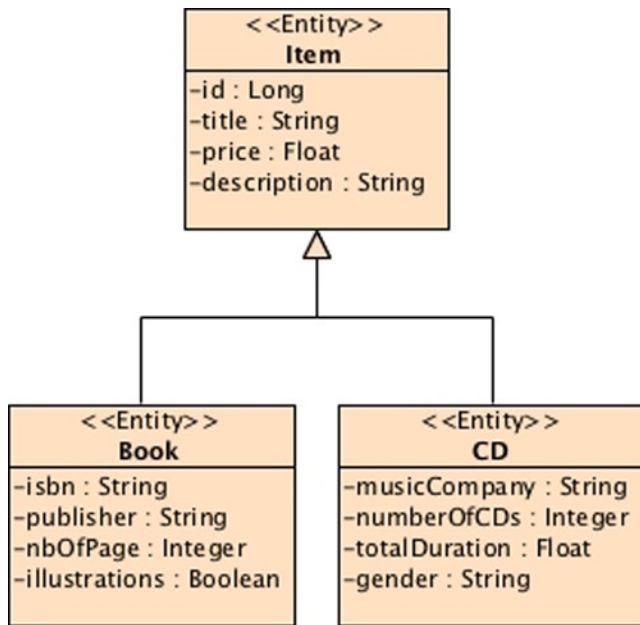
Figure 5-21. Inheritance hierarchy between CD, Book, and Item
