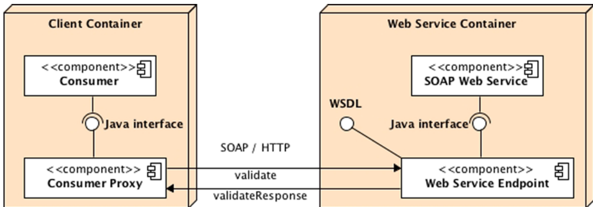
Figure 14-5. A consumer invoking a web service through a proxy
