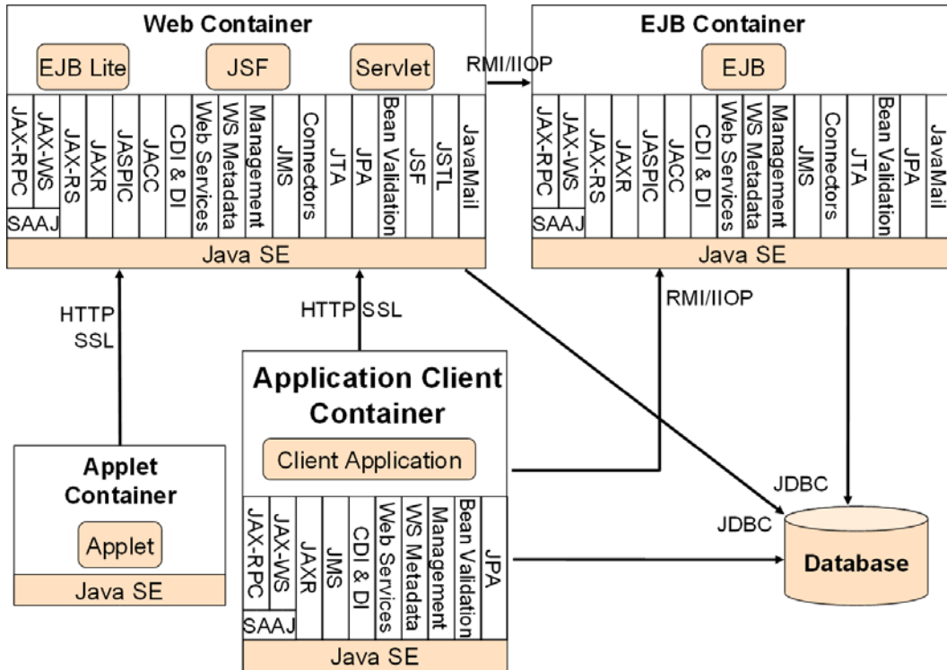
Figure 1-2. Services provided by containers
