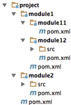
Figure A-5. A project and its modules
