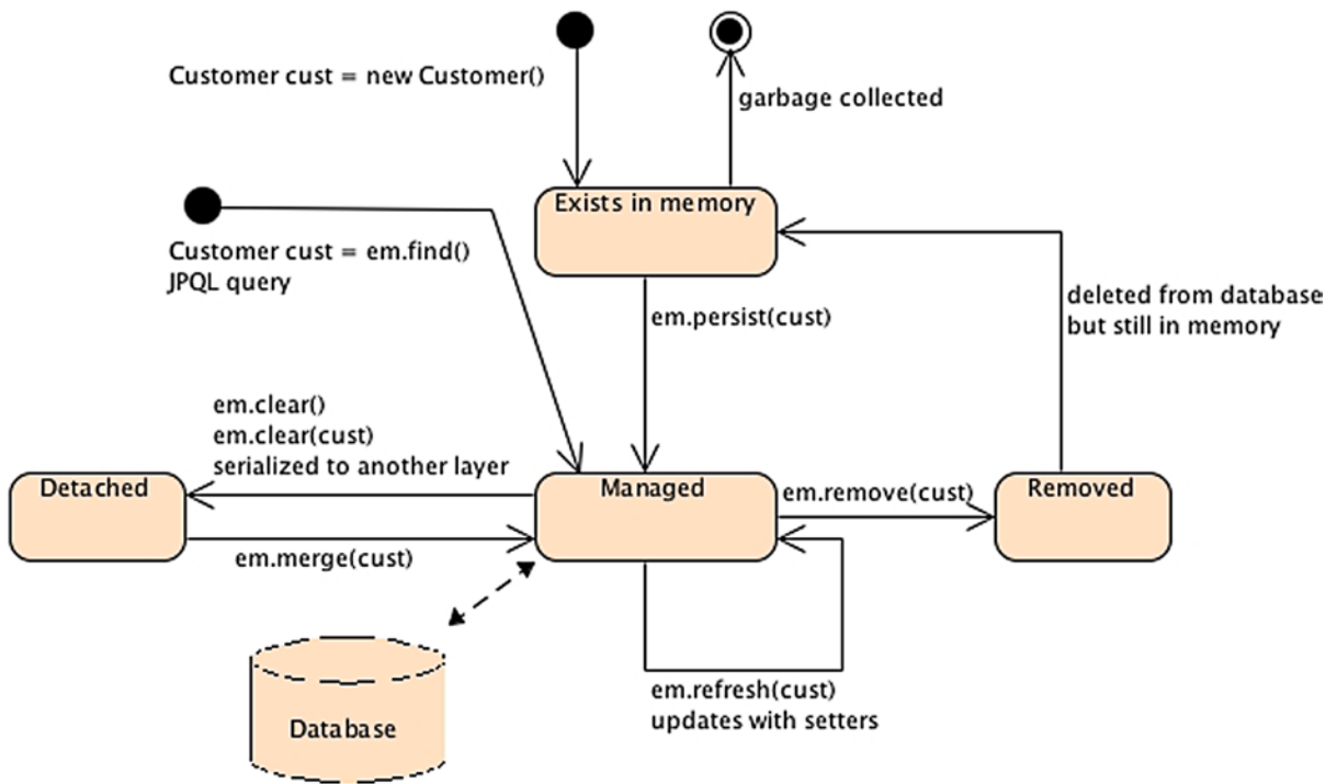
Figure 6-6. Entity life cycle
