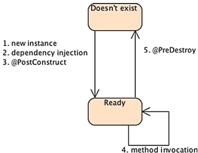
Figure 8-1. Stateless and singleton bean life cycle
