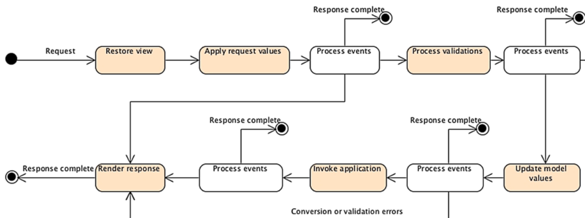
Figure 10-6. The JSF life cycle
