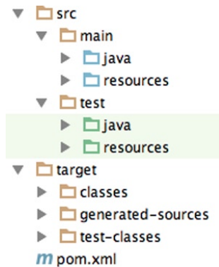
Figure A-3. Standard Maven directory structure
