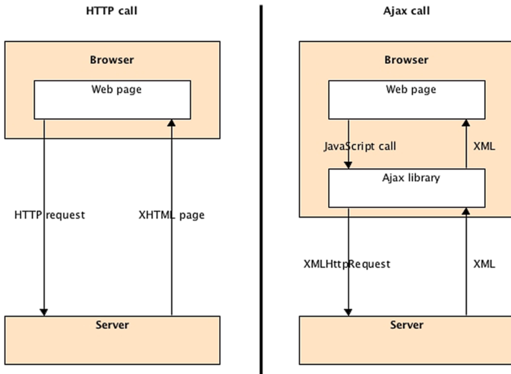
Figure 11-7. Plain HTTP calls vs. Ajax HTTP calls
