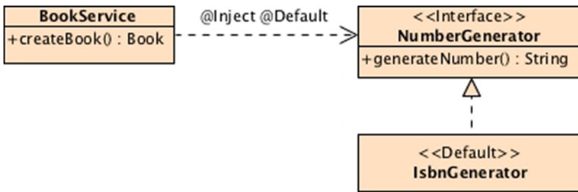
Figure 2-4. Class diagram with @Default injection
