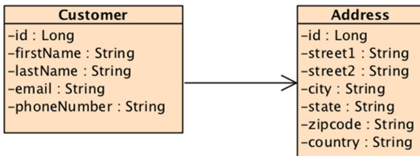
Figure 5-10. A unidirectional association between Customer and Address
