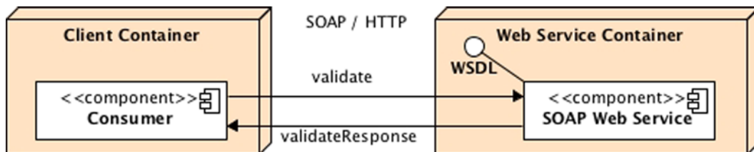
Figure 14-3. A consumer invoking a SOAP web service
