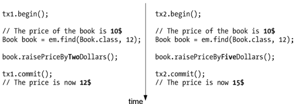
Figure 6-4. Transactions one (tx1) and two (tx2) updating the price of a book concurrently
