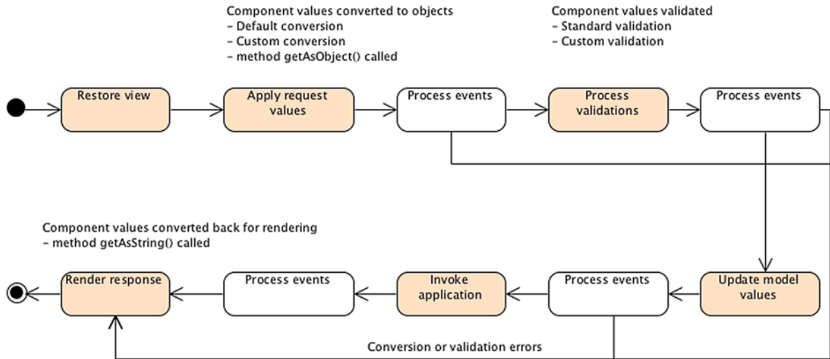
Figure 11-6. Conversion and validation during page life cycle
