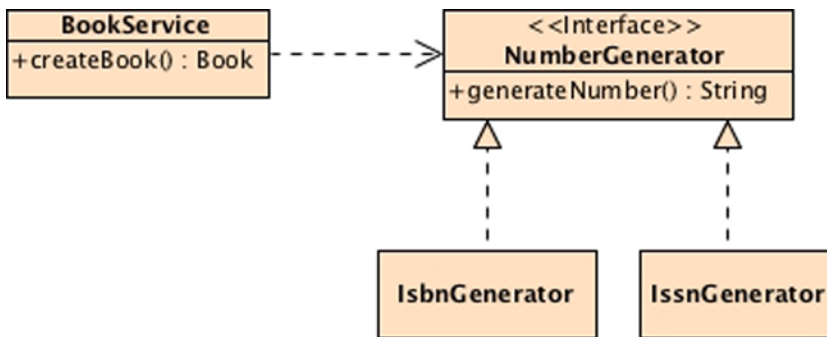
Figure 2-3. Class diagram with the NumberGenerator interface and implementations
