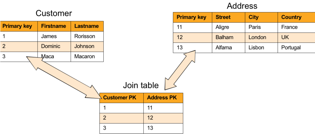
Figure 5-9. A relationship using a join table
