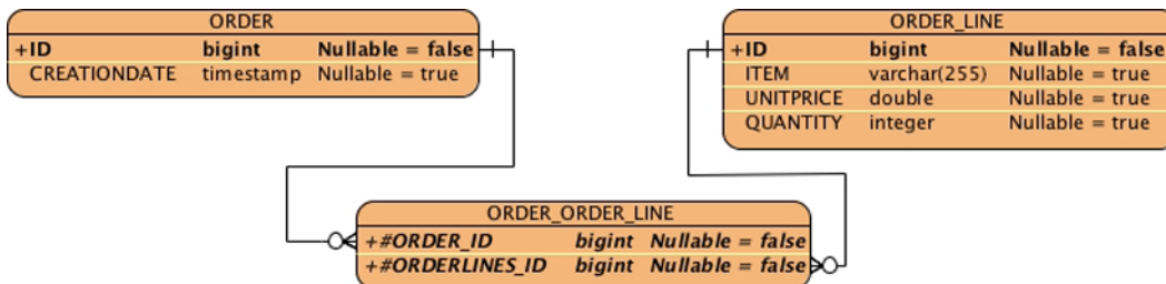
Figure 5-16. Join table between ORDER and ORDER_LINE
