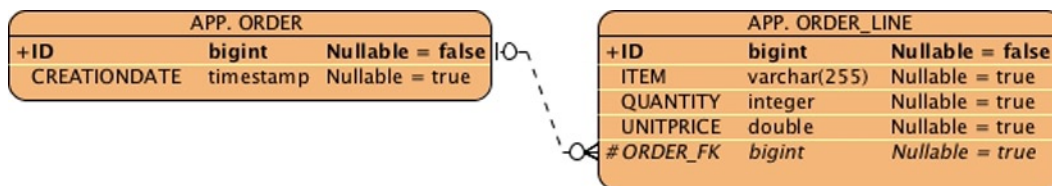
Figure 5-17. Join column between Order and Order_Line
