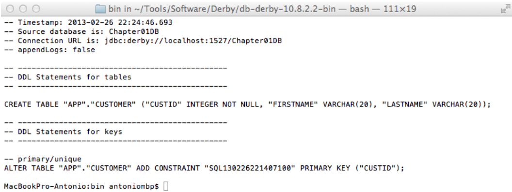
Figure A-9. dblook output of the Chapter01DB database
