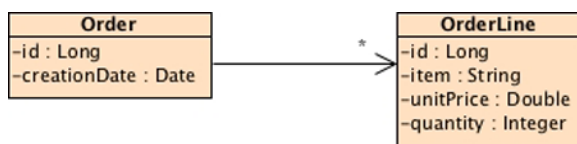
Figure 5-15. One order has several lines
