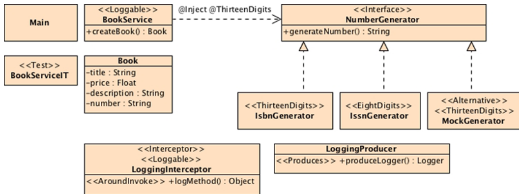
Figure 2-7. Putting It All Together
