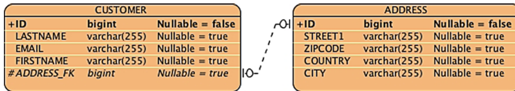
Figure 6-2. CUSTOMER and ADDRESS tables
