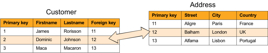
Figure 5-8. A relationship using a join column
