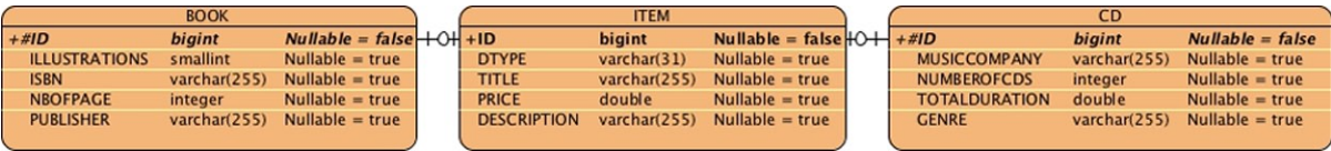
Figure 5-25. Mapping inheritance with a joined-subclass strategy
