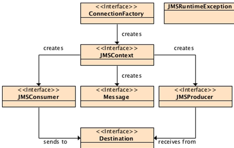
Figure 13-9. JMS Simplified API
