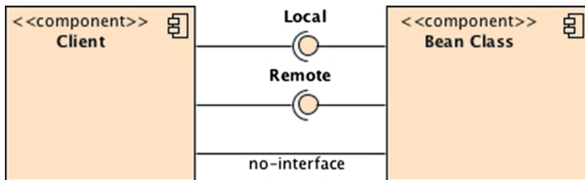
Figure 7-2. Bean class has several types of business interfaces
