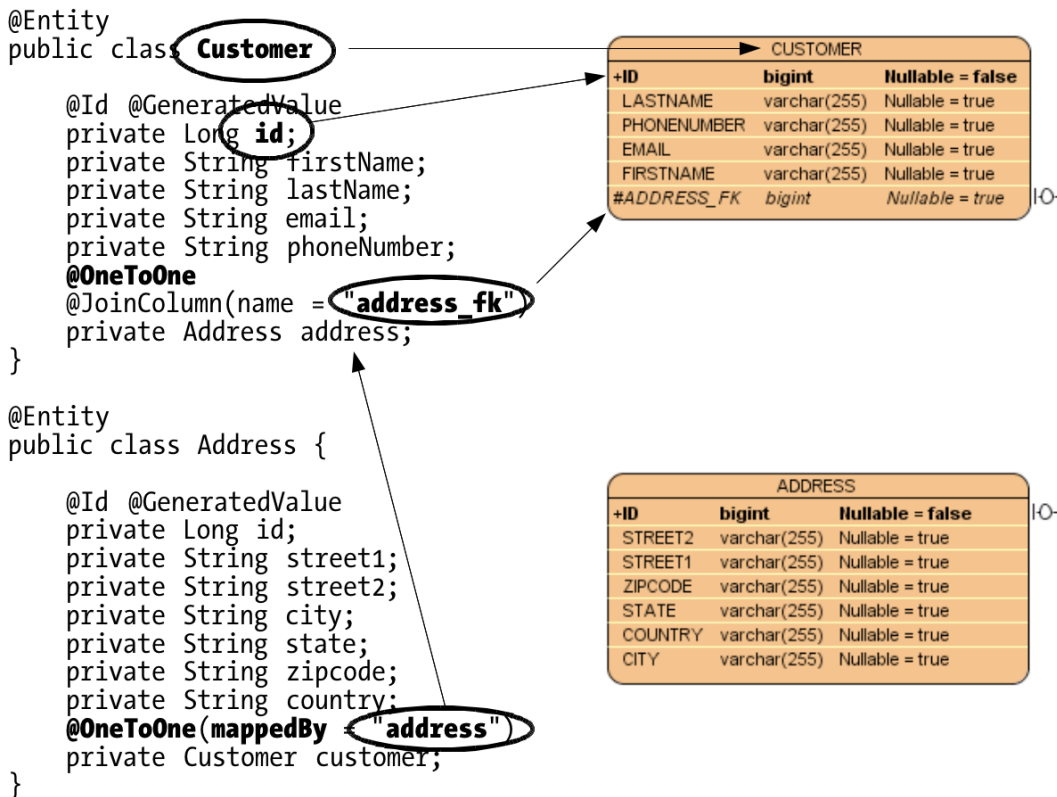
Figure 5-13. Customer and Address code with database mapping
