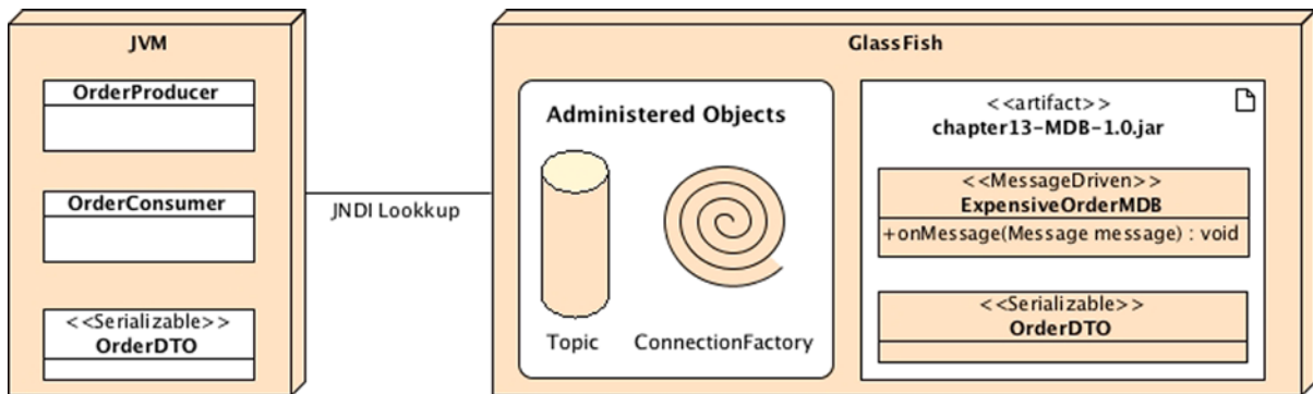
Figure 13-13. Putting It All Together
