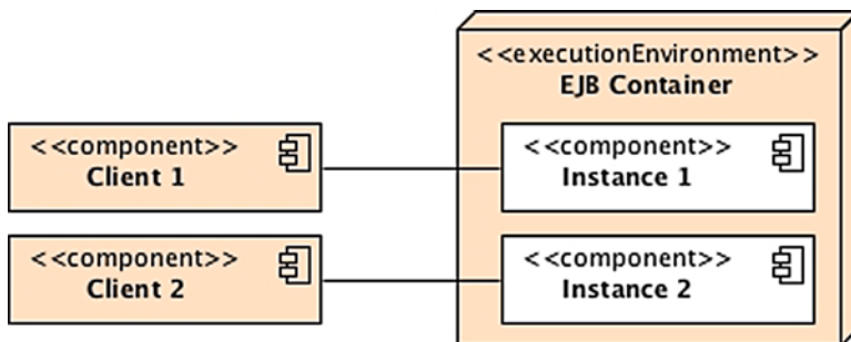
Figure 7-5. Clients accessing stateful beans
