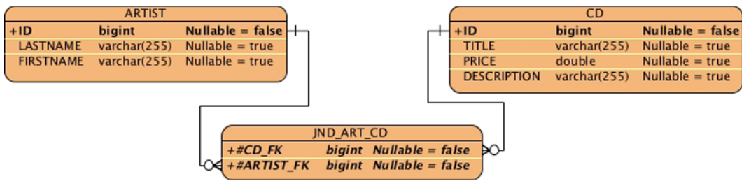
Figure 5-18. Artist, CD, and the join table
