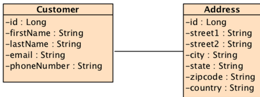
Figure 5-11. A bidirectional association between Customer and Address
