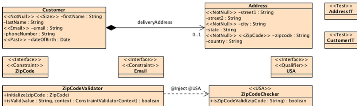
Figure 3-2. Putting it all together
