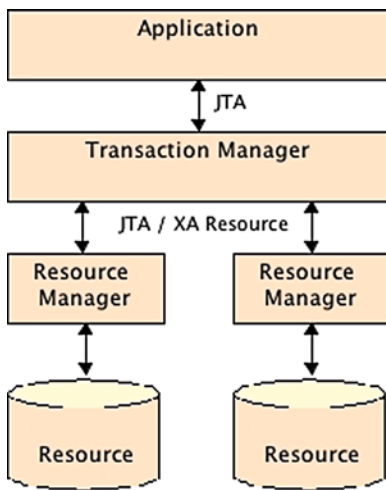
Figure 9-2. An XA transaction involving two resources
