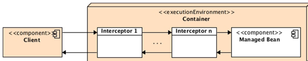
Figure 2-2. A container intercepting a call and invoking interceptors
