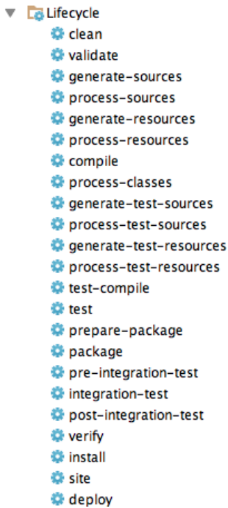
Figure A-6. Project life cycle
