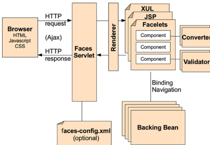
Figure 10-5. JSF architecture
