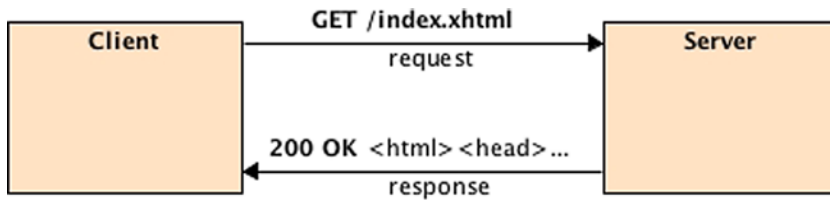
Figure 15-1. HTTP request and response
