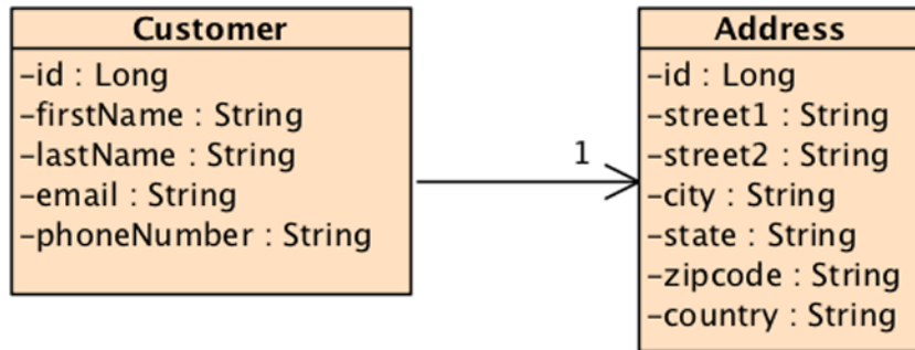
Figure 5-14. One customer has one address
