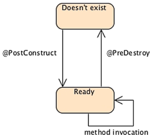
Figure 11-3. The backing bean life cycle
