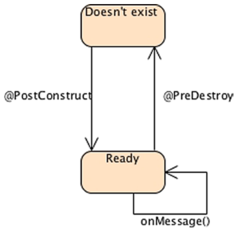
Figure 13-12. MDB life cycle
