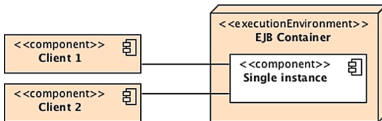
Figure 7-6. Clients accessing a singleton bean
