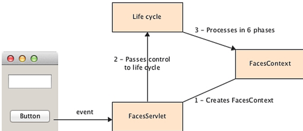
Figure 11-2. The FacesServlet interactions
