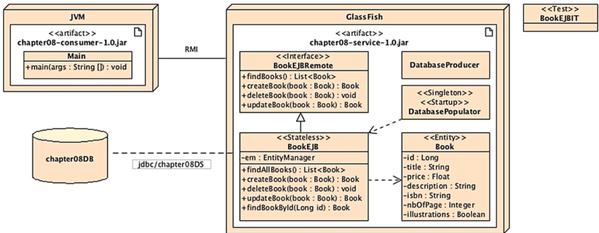
Figure 8-4. Putting it all together
