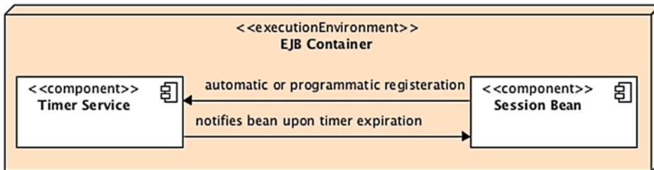
Figure 8-3. Interaction between the timer service and the session bean
