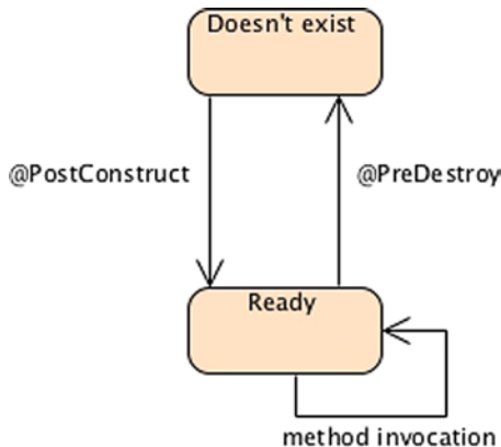
Figure 14-4. SOAP web service life cycle
