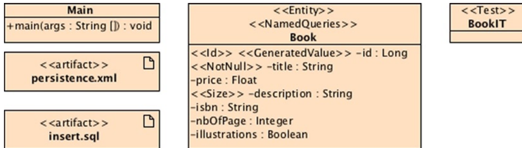
Figure 4-4. Putting it all together
