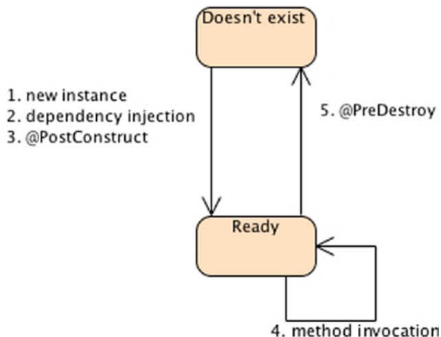
Figure 2-1. Managed Bean life cycle
