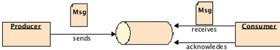
Figure 13-11. A consumer acknowledging a message
