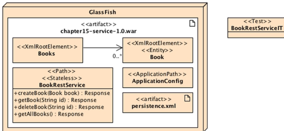
Figure 15-4. Putting It All Together
