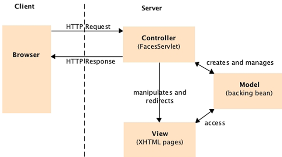
Figure 11-1. The MVC design pattern
