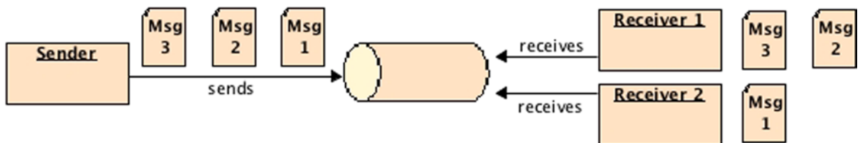
Figure 13-4. Multiple receivers
