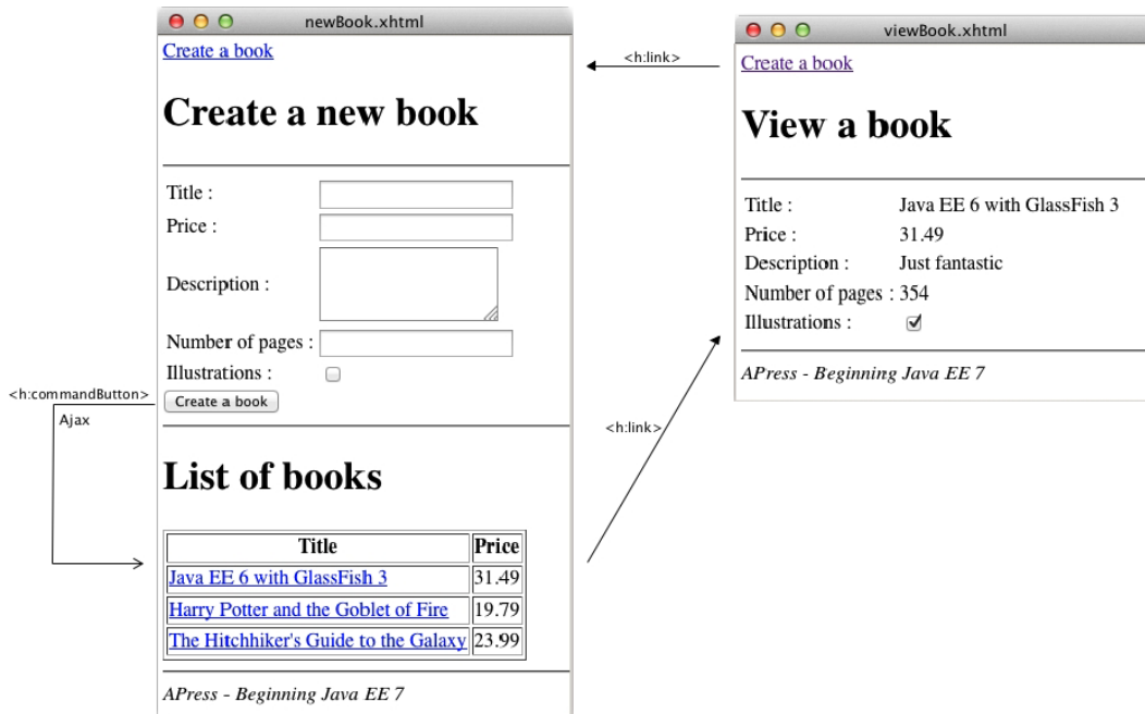
Figure 11-8. Navigating between newBook.xhtml and viewBook.xhtml
