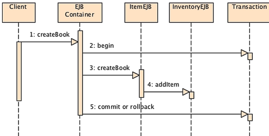
Figure 9-5. The container handles the transaction
