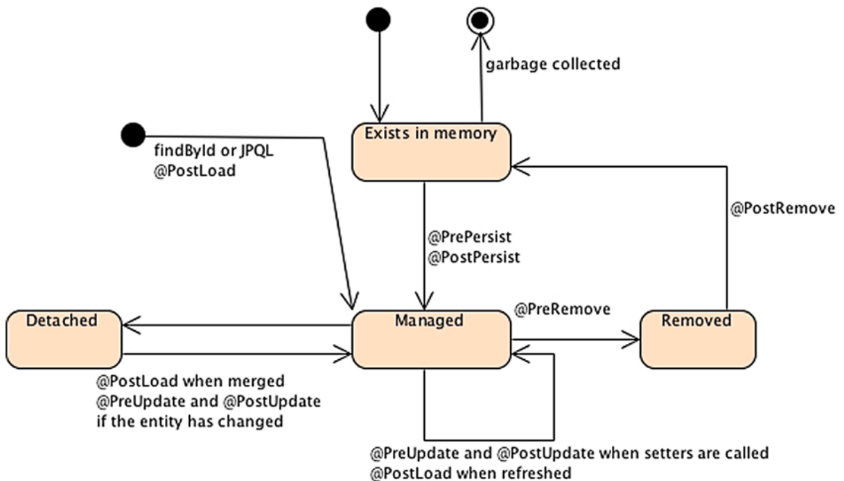
Figure 6-7. Entity life cycle with callback annotations
