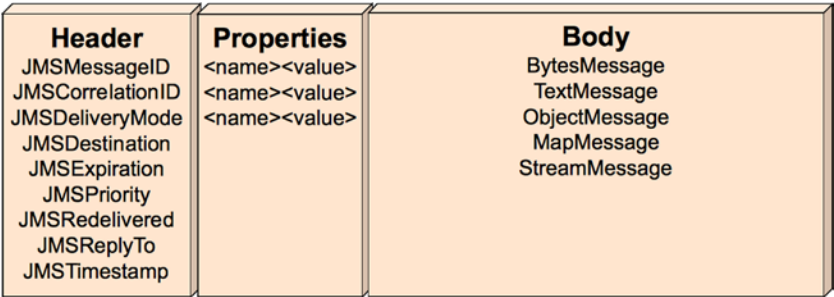
Figure 13-8. Structure of a JMS message
