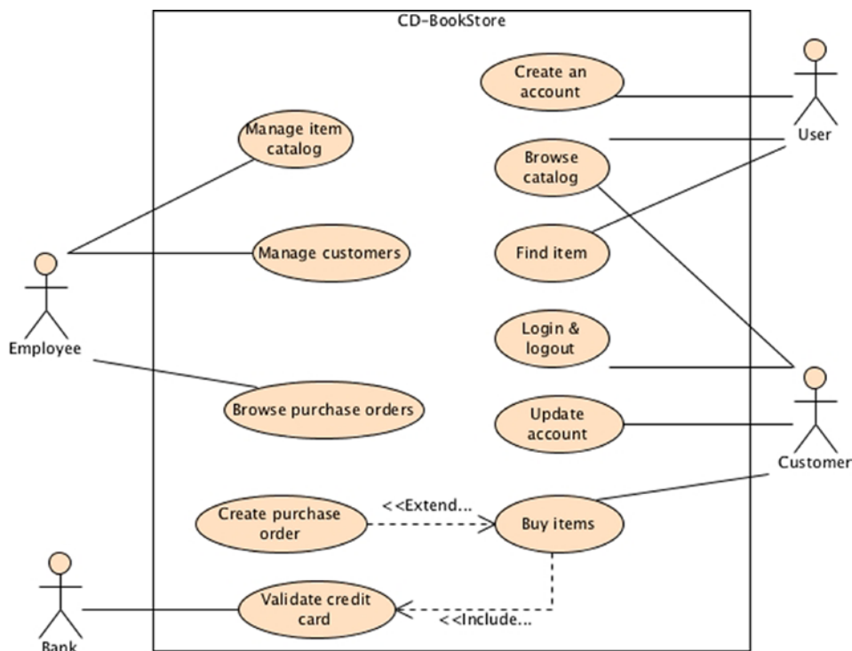
Figure 1-6. Use case diagram of the CD-BookStore application
