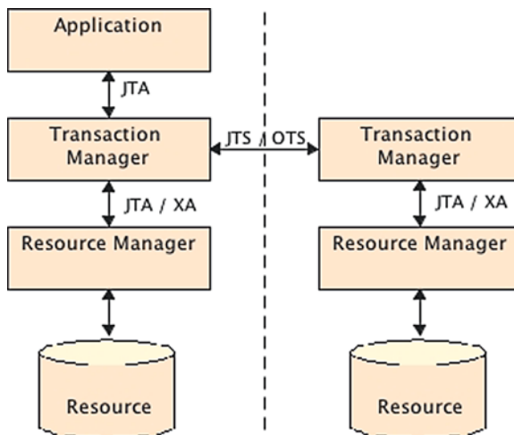
Figure 9-4. A distributed XA transaction
