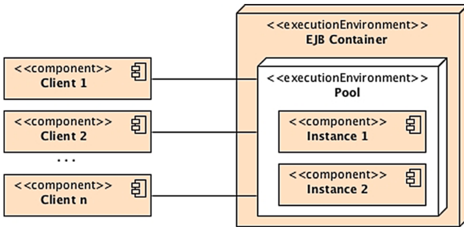
Figure 7-4. Clients accessing stateless beans in a pool
