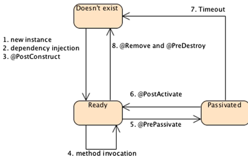
Figure 8-2. Stateful bean life cycle
