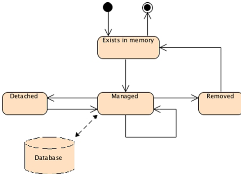
Figure 4-3. The life cycle of an entity
