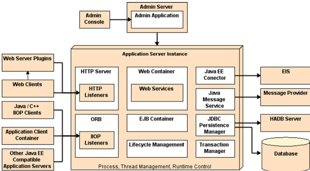
Figure A-11. Functional parts of GlassFish
