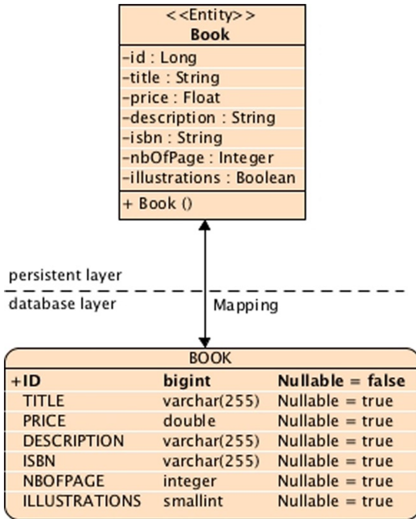
Figure 4-1. Data synchronization between the entity and the table
