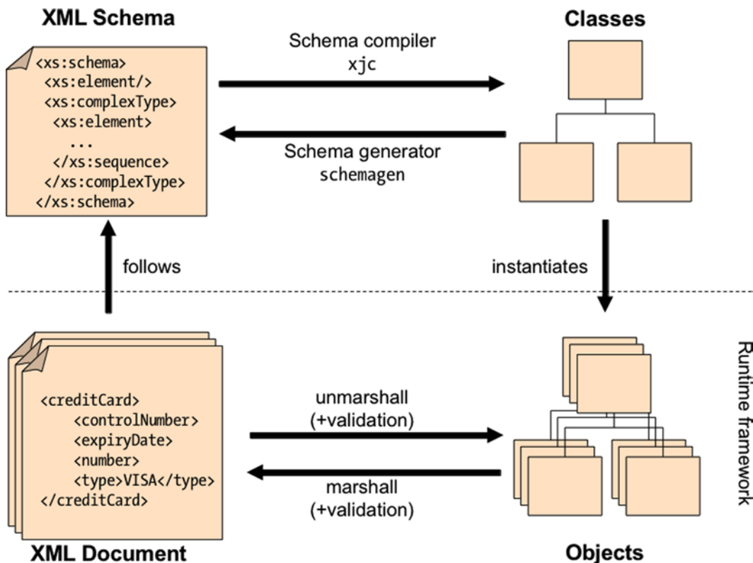
Figure 12-2. JAXB architecture
