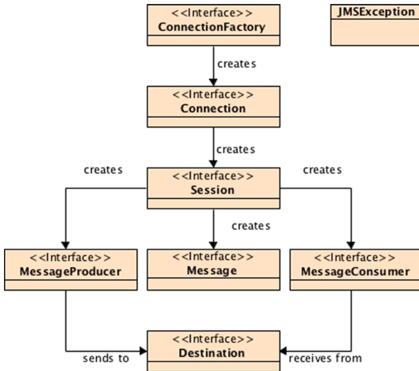
Figure 13-7. JMS Classic API
