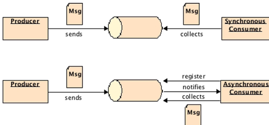
Figure 13-10. Synchronous and asynchronous consumers
