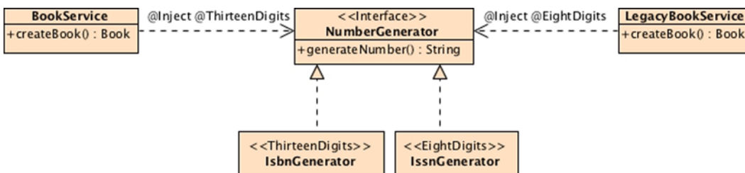
Figure 2-5. Services using qualifiers for non-ambiguous injection
