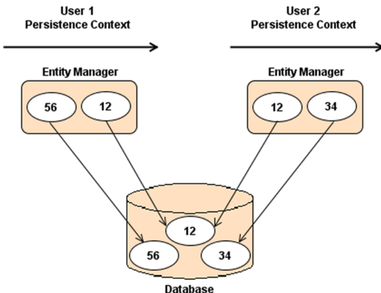
Figure 6-1. Entities living in different users’ persistence context
