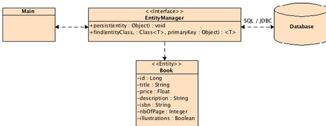
Figure 4-2. The entity manager interacts with the entity and the underlying database
