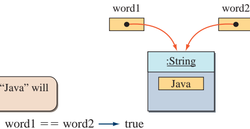
Figure 5.6 Difference between using and not using the new operator for String .
