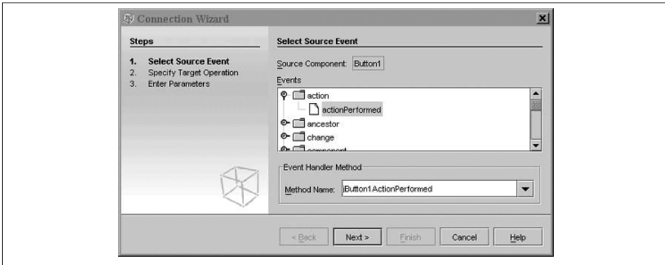
Figure 22-4. Selecting a source event in the Connection Wizard
